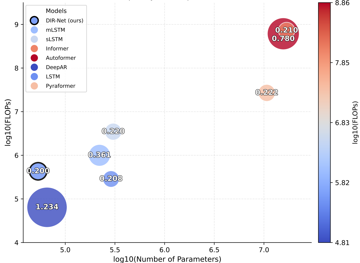
Model Complexity vs Computation vs MSE
